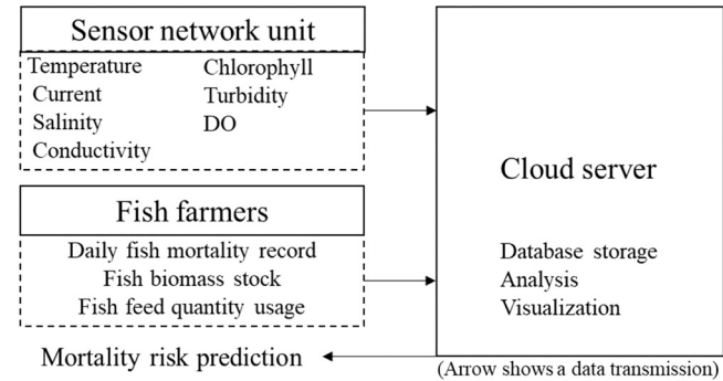
Fig. 4. Diagram of the real-time data collection and transferring scheme in this study.
